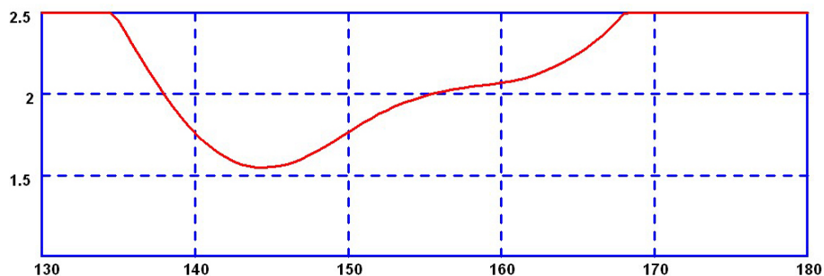
Typical VSWR*
