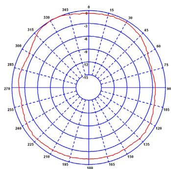
Typical H-Plane
